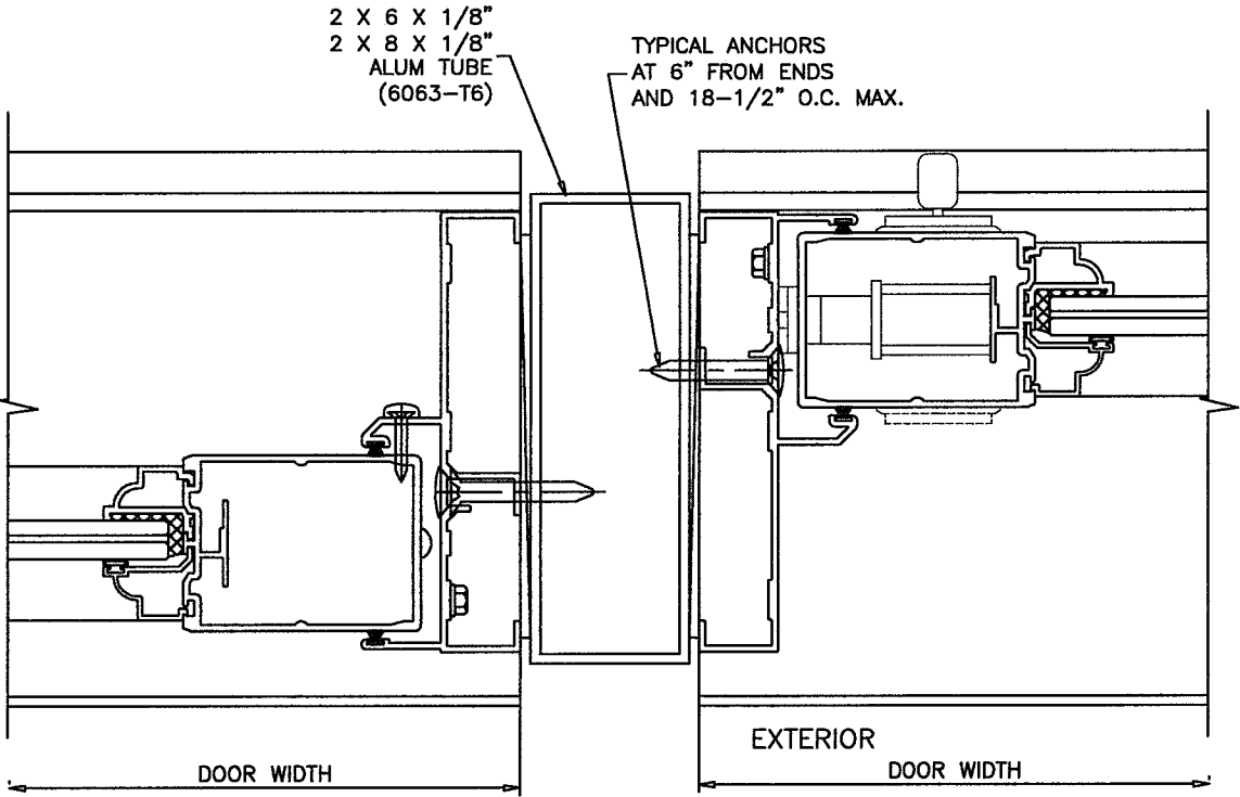
UNCLIPPED MULLION
